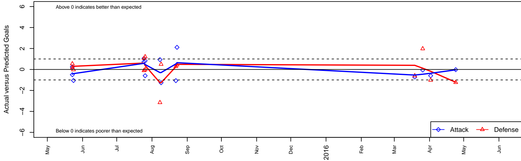
FC Golden State 00 PDA B99 Dots are actual minus expected GF (blue circles) and GA (red triangles). Blue line is smoothed change in attack strength. Red is smoothed change in defense strength.
